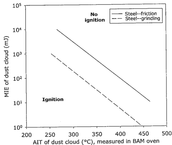
Figure 2 Boundaries for steel surface frictional and impact ignition of dust clouds (from Babrauskas, 2003)
